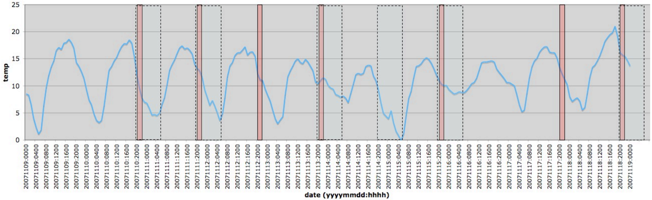
Appendix 2. Mean temperature for Turangi 2 Ews observation station. Bat transect line sampling periods seen as red shaded areas, ABM sampling periods seen as light blue shaded areas with dashed outlines.
